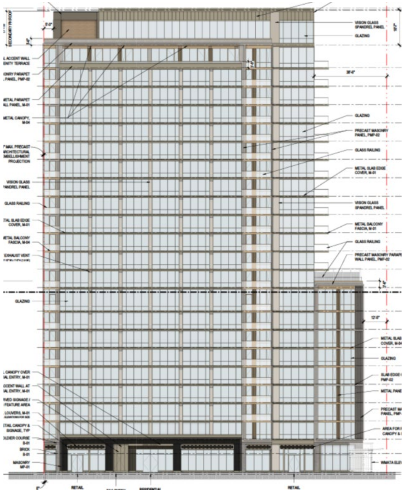
Figure 15-- North Elevation
