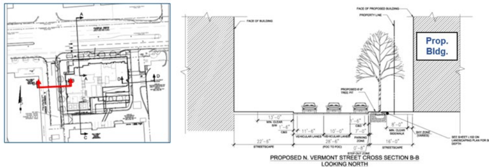
Figure 22. Proposed North Vermont Street Cross-Section (Facing North)
