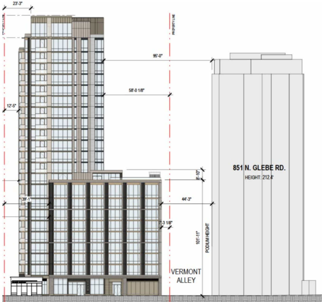
Figure 16 Comparative elevation showing building distance to Continental Condos
