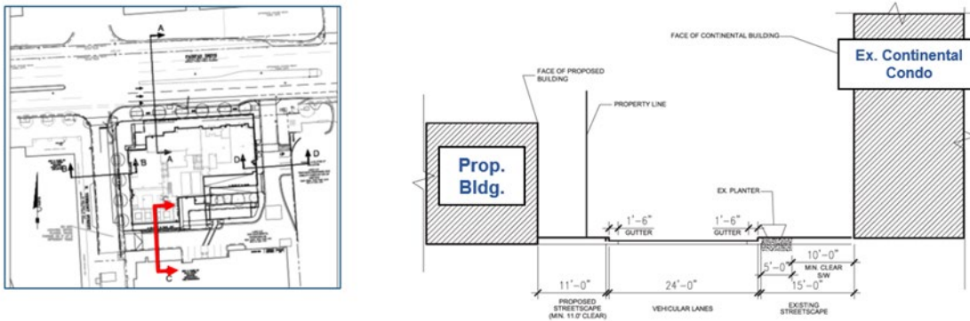
Figure 24. Proposed Vermont Alley Cross-Section (Facing West)
