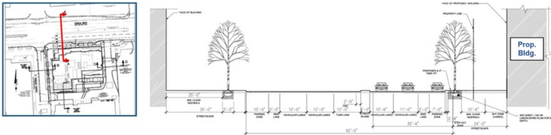
Figure 21. Proposed Fairfax Drive Cross-Section (Facing East)
