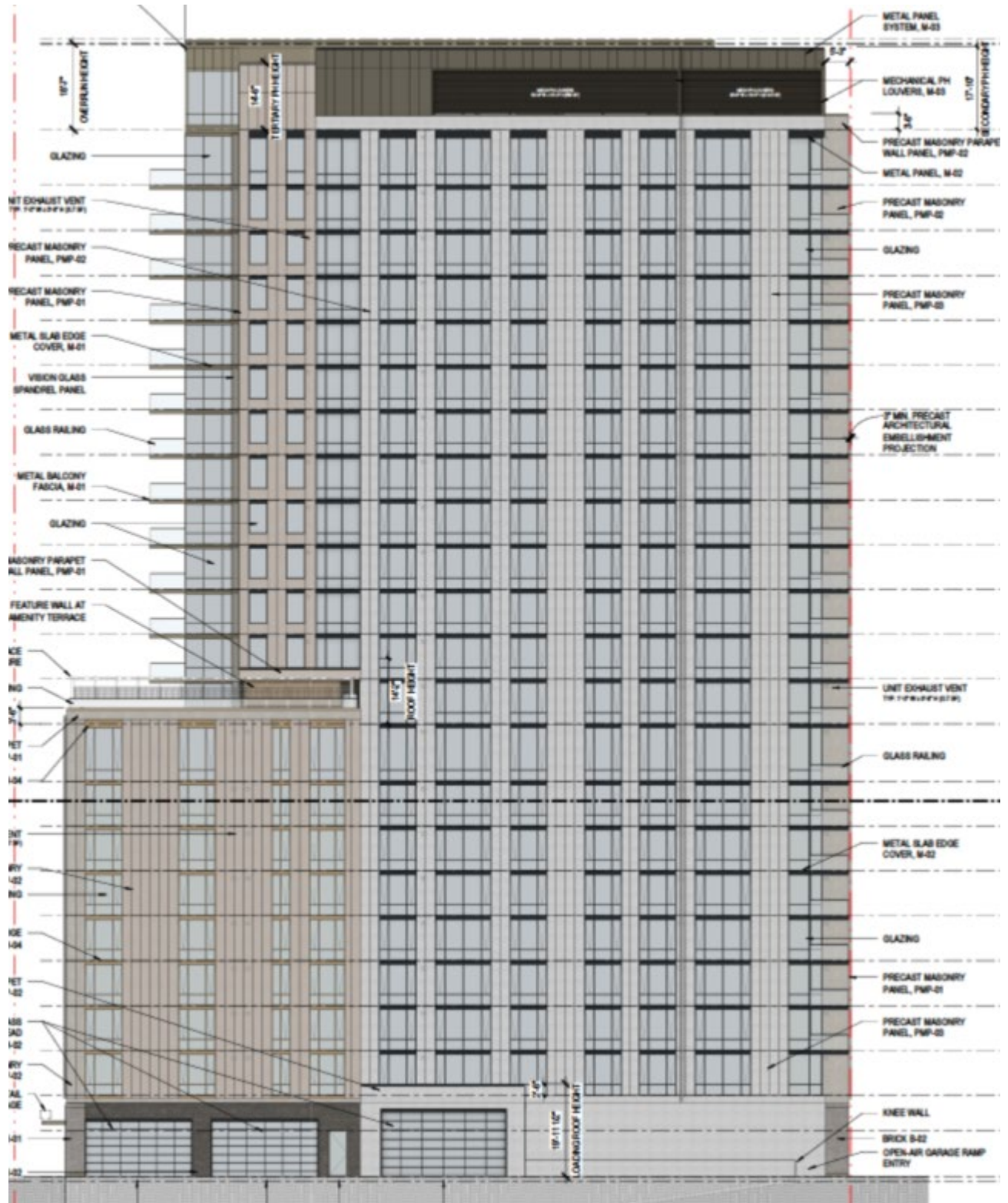
Figure 13-- South elevation
