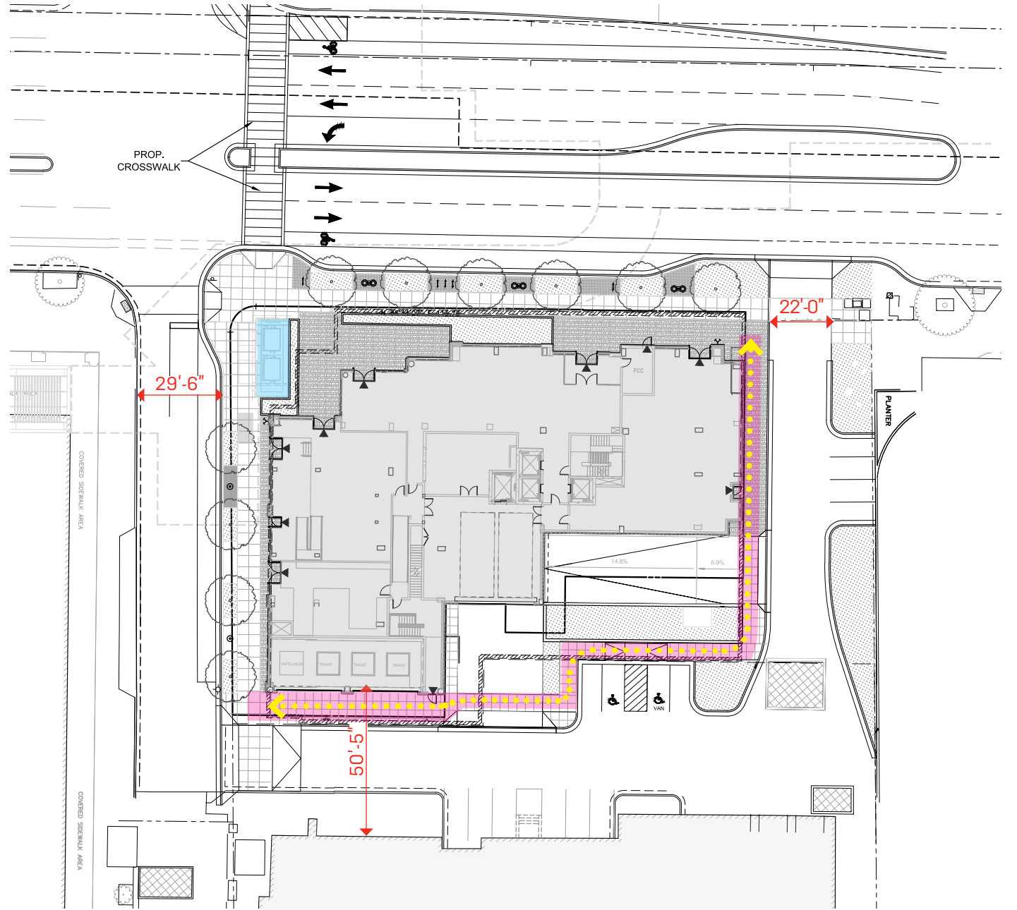
PROPOSED SITE AREA PLAN
