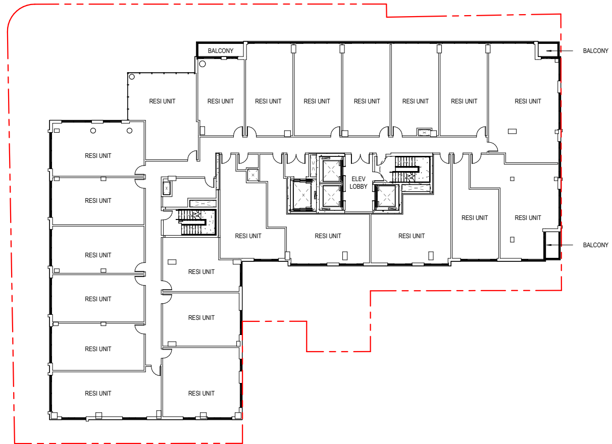
1 | 4.1 - FLOOR PLAN - LEVEL 04 THRU 09
