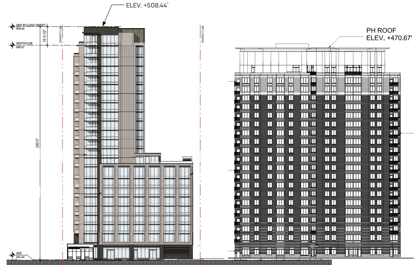
CURRENT PROPOSED WEST ELEVATION
