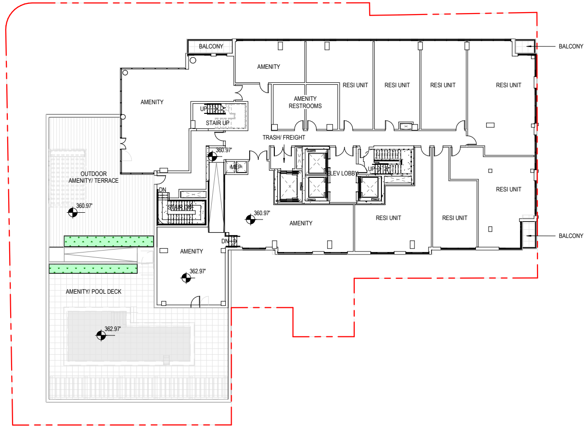
1 | 4.1 - FLOOR PLAN - LEVEL 10 1/16" = 1'-0" 0 8' 16' 32'
