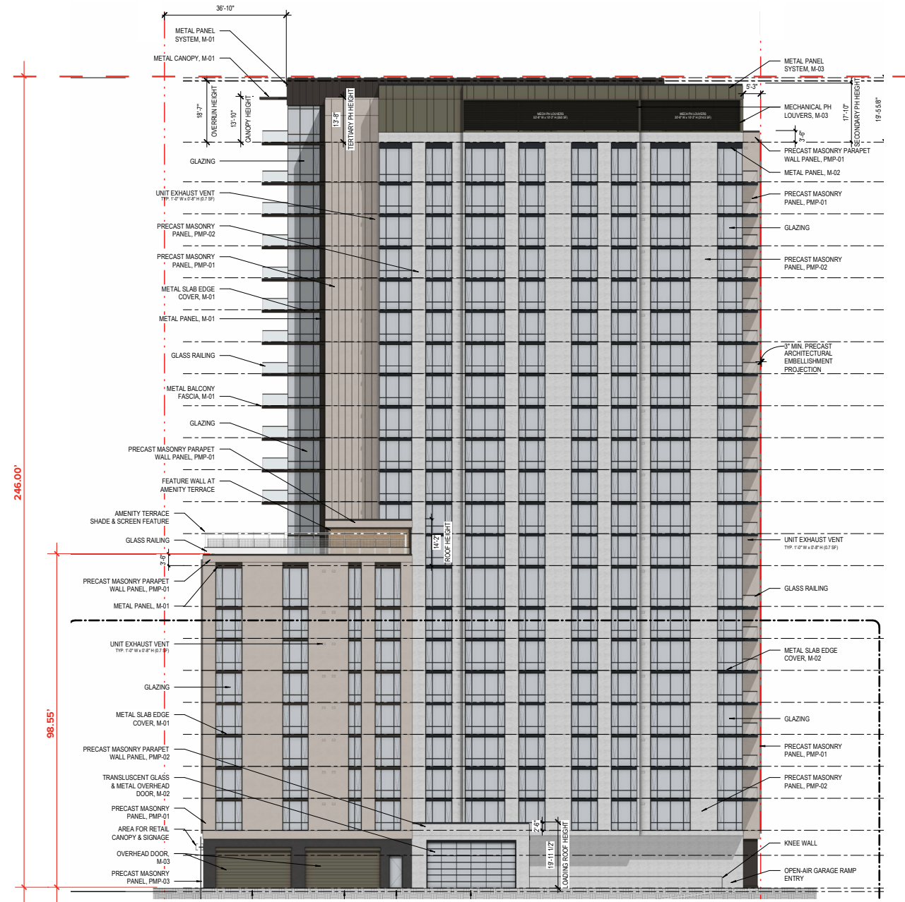
CURRENT PROPOSED SOUTH ELEVATION
