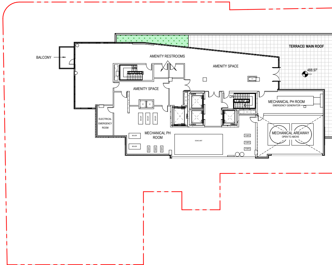
1 | 4.1 - FLOOR PLAN - LEVEL PENTHOUSE
