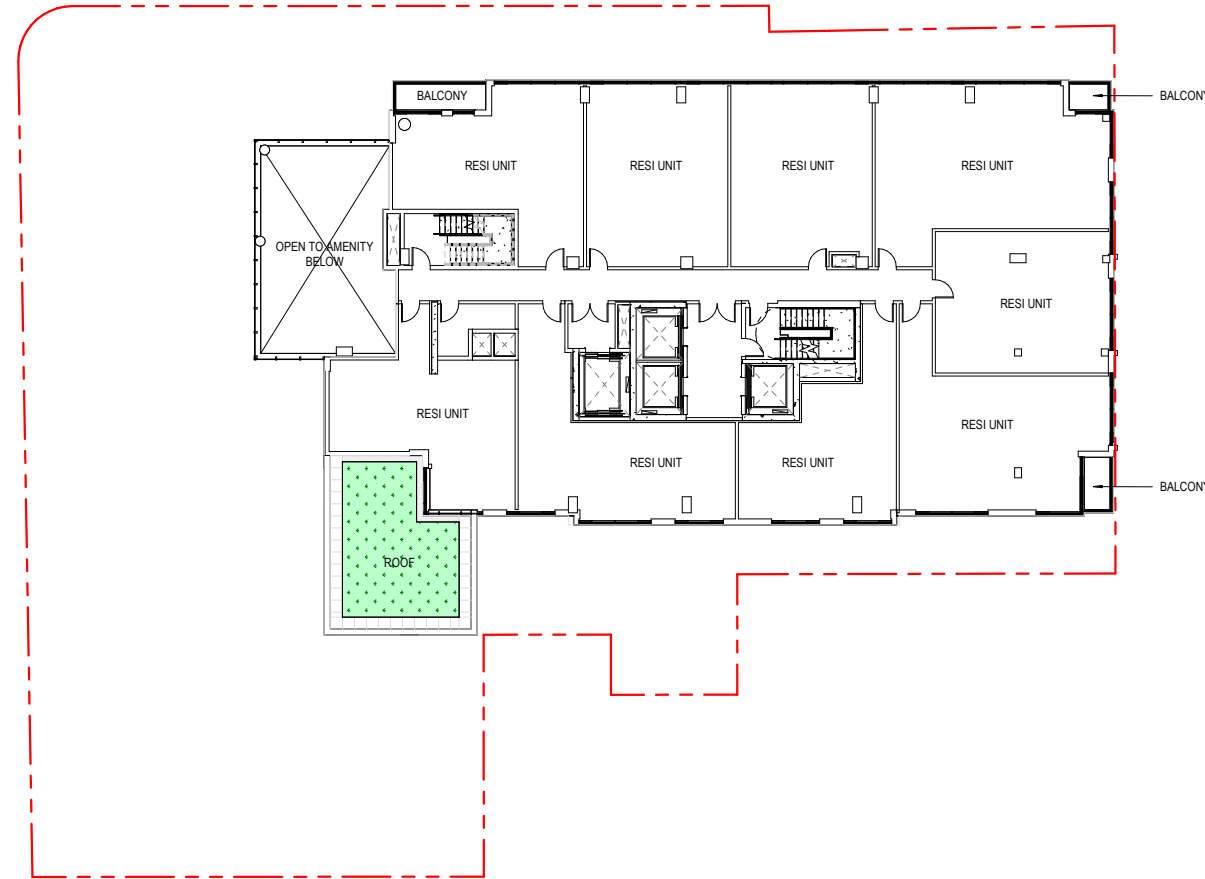
2 | 4.1 - FLOOR PLAN - LEVEL 11 1/16" = 1'-0" 0 8' 16' 32'
