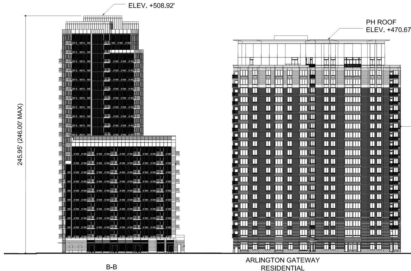
PREVIOUSLY APPROVED WEST ELEVATION
