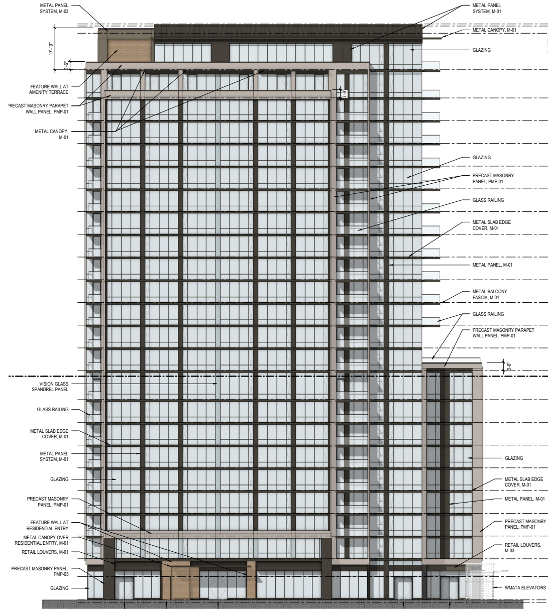
CURRENT PROPOSED NORTH ELEVATION
