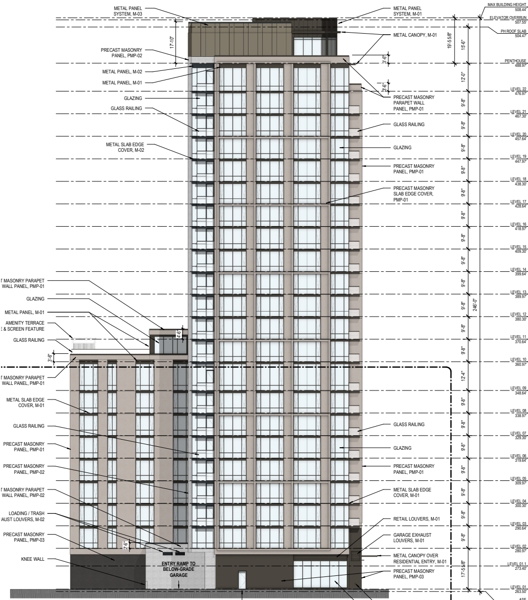
CURRENT PROPOSED EAST ELEVATION
