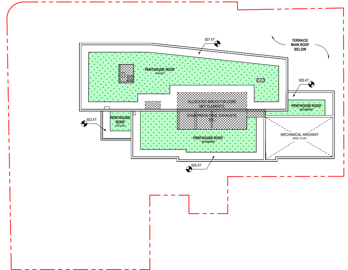
2 | FLOOR PLAN - PENTHOUSE ROOF
