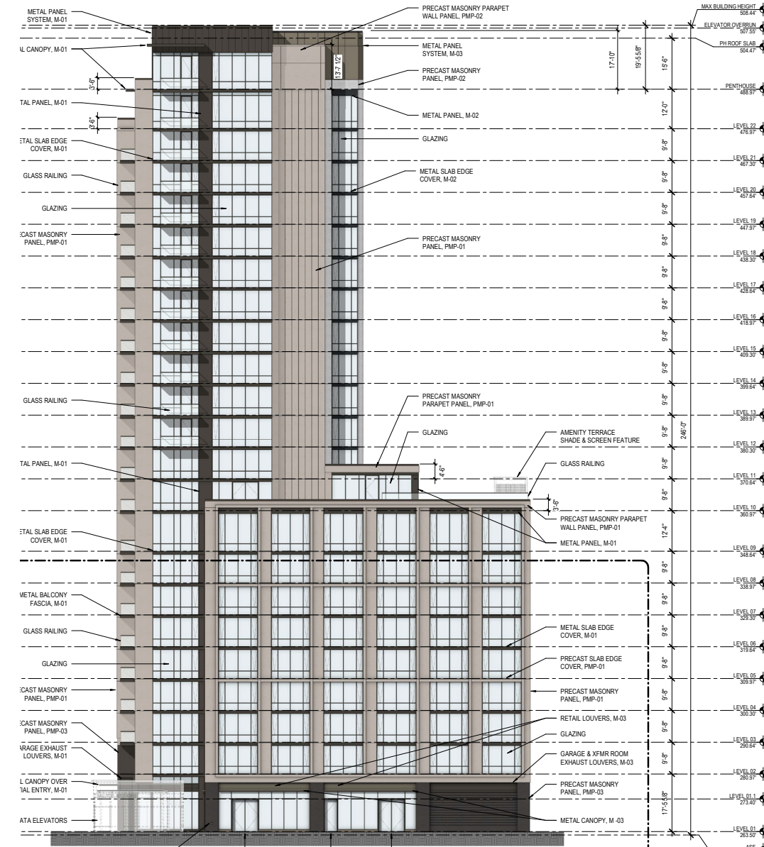
CURRENT PROPOSED WEST ELEVATION
