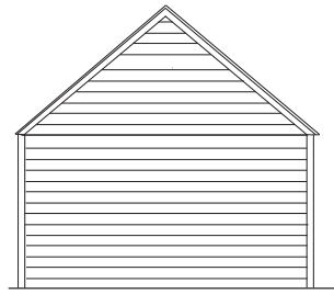
PROPOSED NORTH ELEVATION
