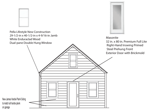
PROPOSED ALTERNATE SOUTH ELEVATION
