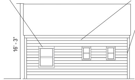
PROPOSED WEST ELEVATION
