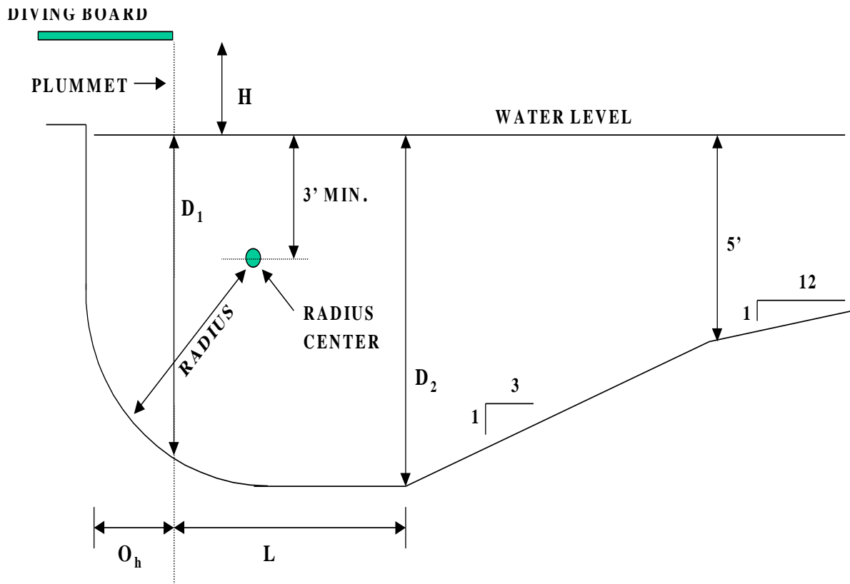
Figure 1. Cross-Sectional Diagram of Swimming Pool Illustrating Distances Referenced in Table II.
