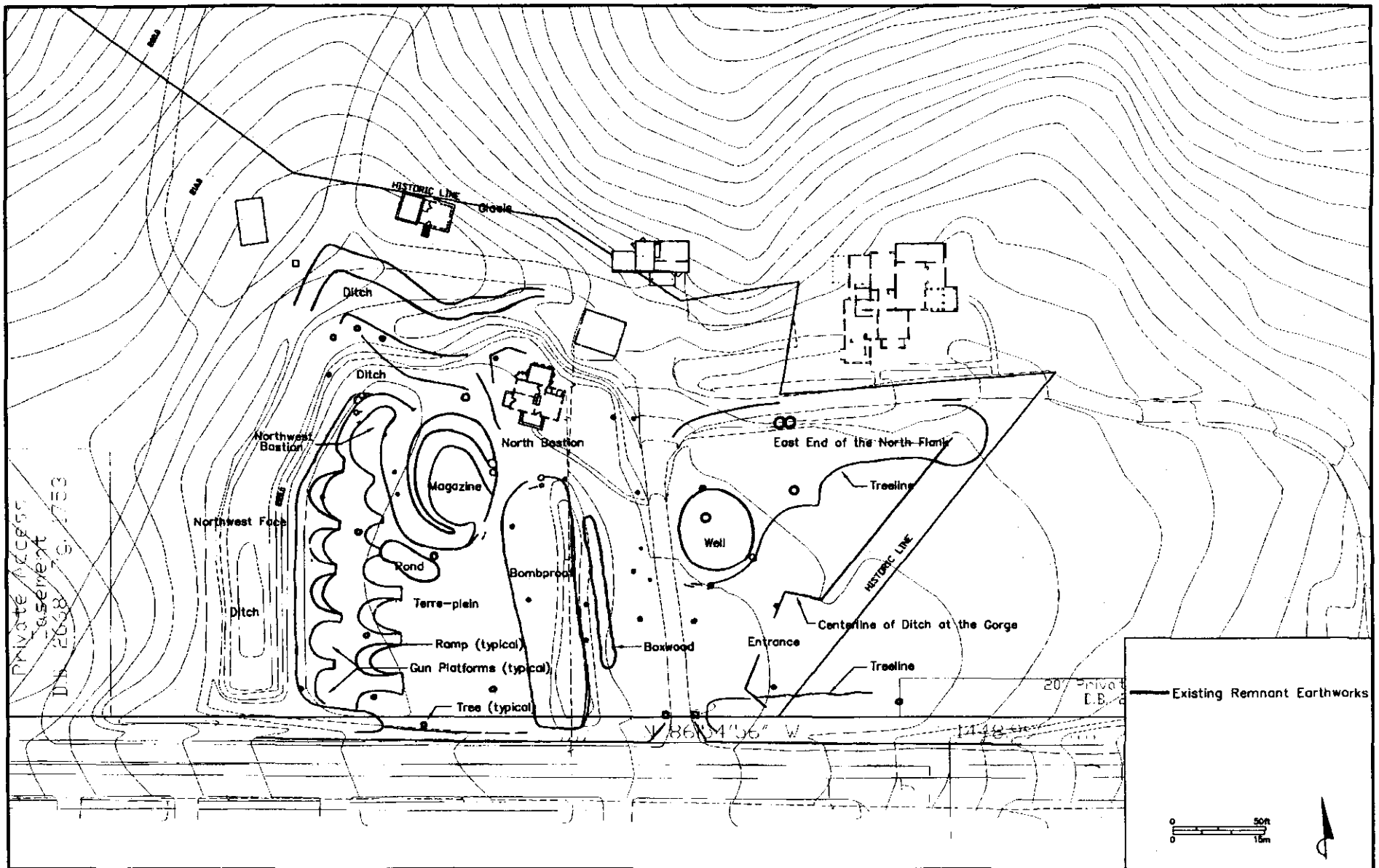
Figure 9. Existing remnant earthworks at Fort C. F. Smith Park.
