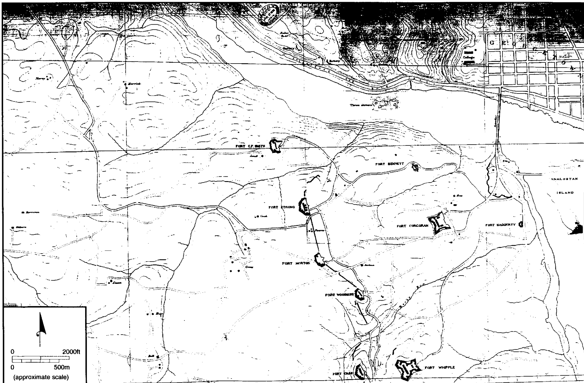
Figure 5. Detail of topographic map showing the northwest portion of the Arlington Line (Barnard, 1871).
