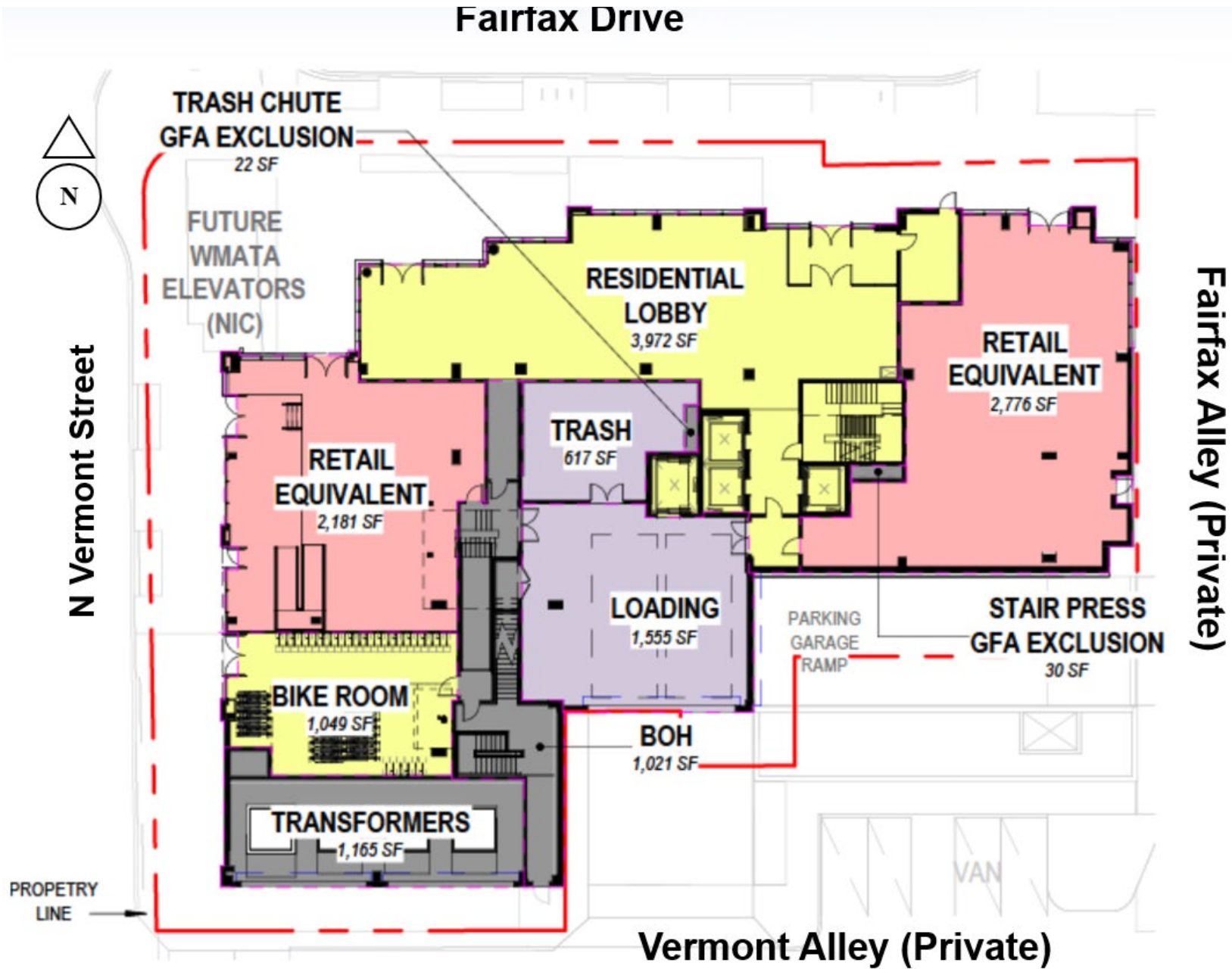
Figure 1-- ground floor layout
