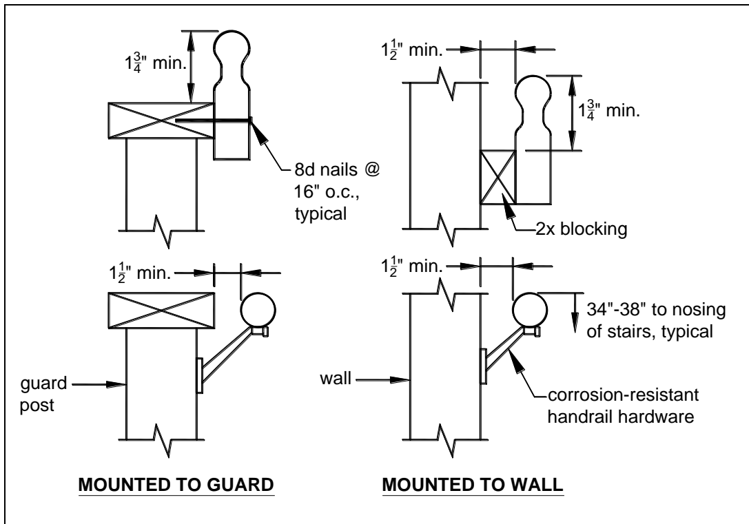
FIGURE 40: HANDRAIL REQUIREMENTS
