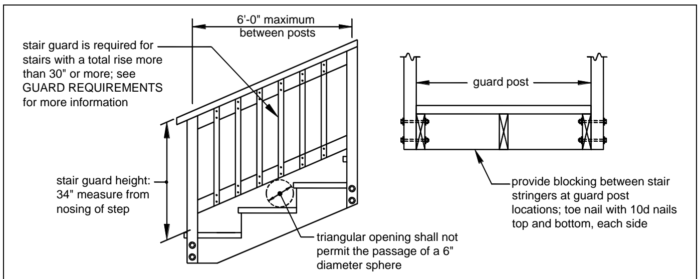
FIGURE 36: STAIR GUARD REQUIREMENTS
