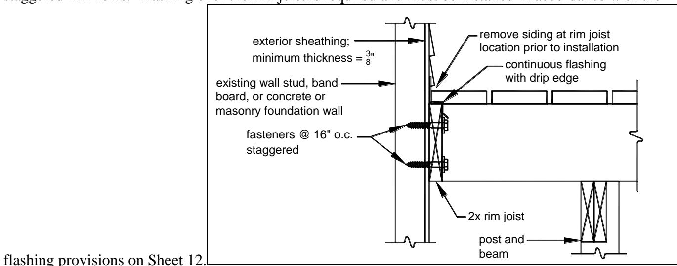
FIGURE 25: ATTACHMENT TO HOUSE LATERAL SUPPORT
