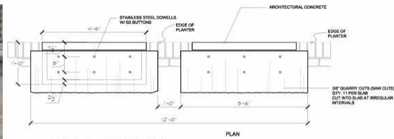
10 PLAN- SECURITY BENCH 3/4" = 1'-0"
