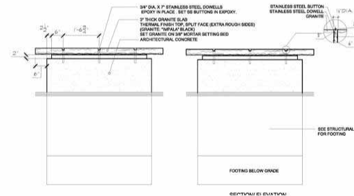
11 ELEVATION- SECURITY BENCH 3/4" = 1'-0"
