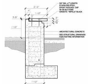
8 SECTION- SECURITY BENCH 3/4" = 1'-0"
